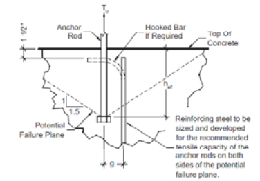
Fig. 9.1.4 The Use of Steel Reinforcement for Developing Anchor Rods
